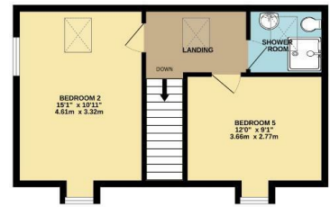
2ND FLOOR 409 sq.ft. (38.0 sq.m.) approx.
